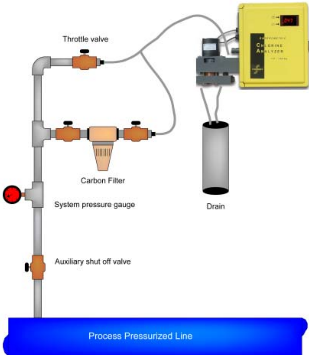
FX-1000p-B Bufferless Chlorine Analyzer
