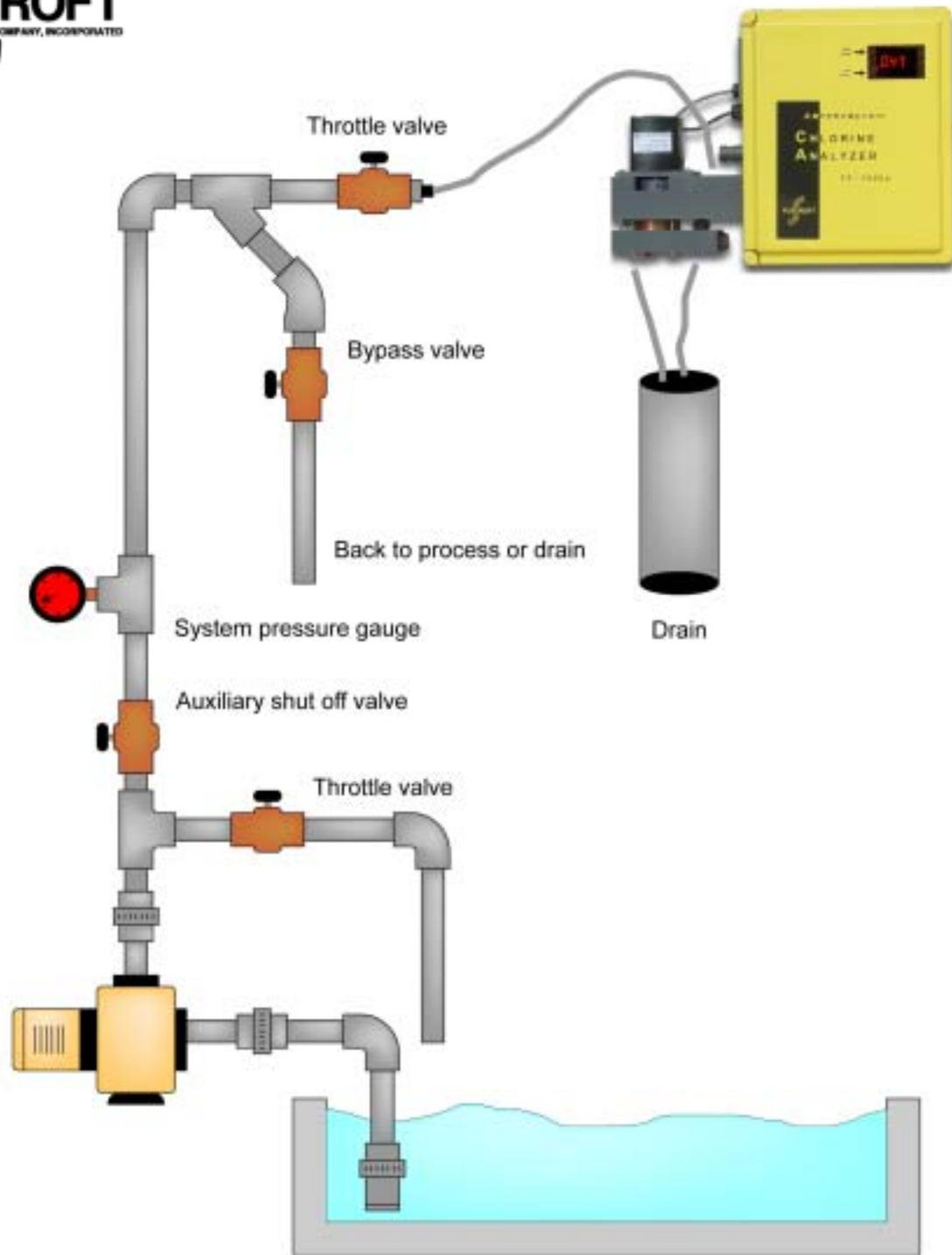
FX-1000p-B Bufferless Chlorine Analyzer
